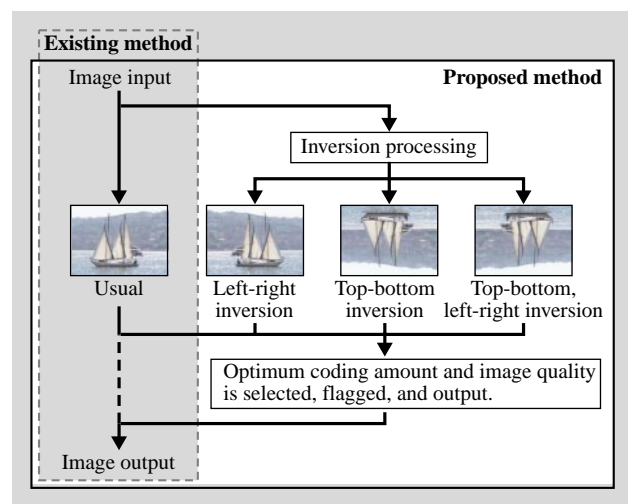
Fig. 6—Overview of H.264/AVC Extended Coding by Picture Inversion.
