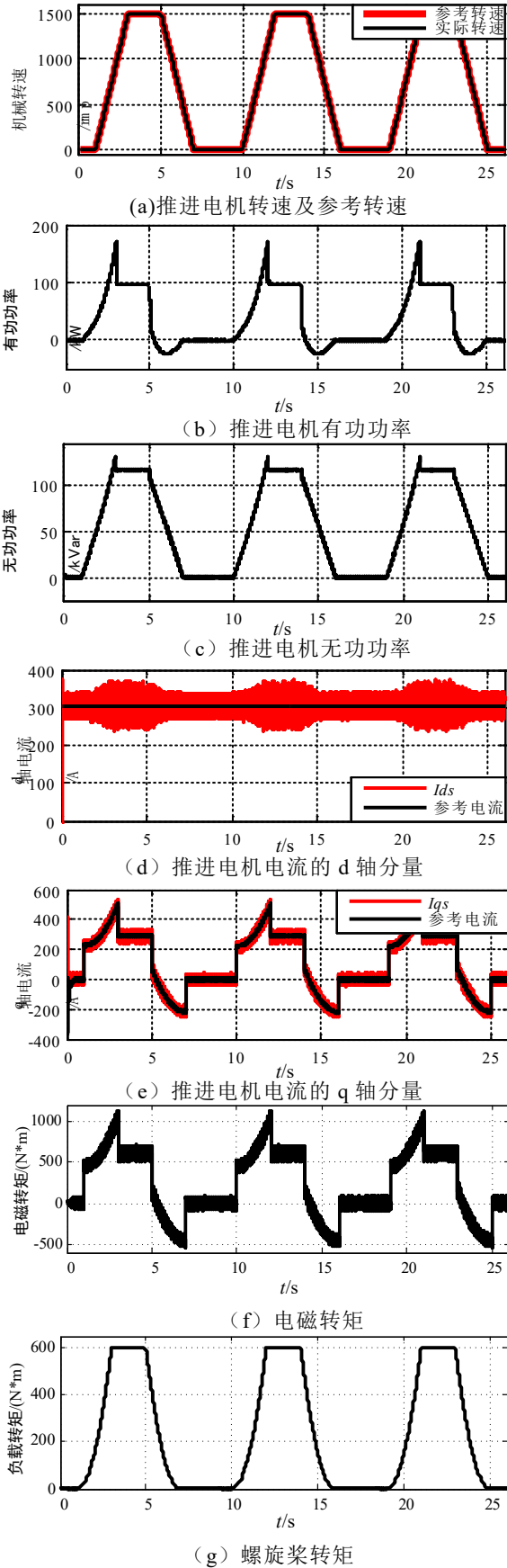
图 10 艏侧推进器仿真结果 Fig.10 Simulation results of bow thruster.
