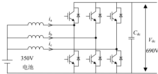
图 3 三相交错并联 DC/DC 变换器电路拓扑 Fig.3 Circuit topology of three-phase interleaved parallel DC/DC converter.
