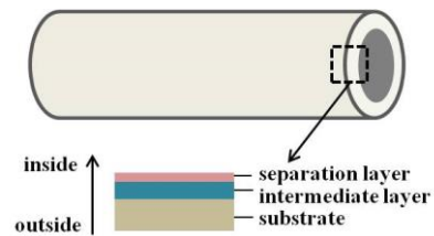
(a) membrane coated on the inner-side of the tube
