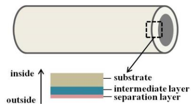
(b) membrane coated on the outer-side of the tube
